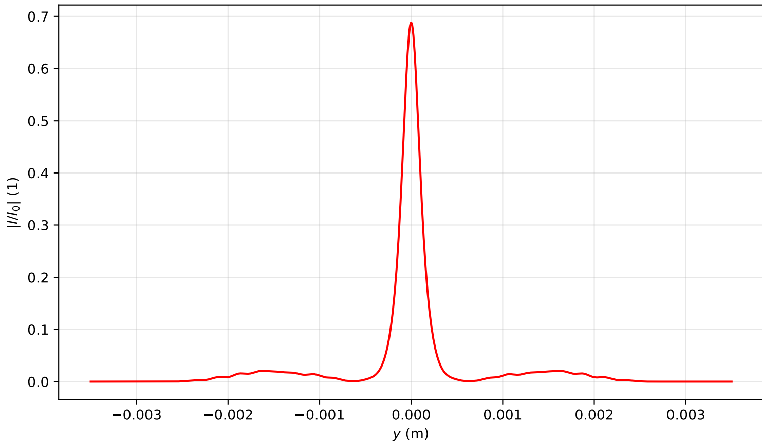
Intensity profile I(x=0, y, z=1.592)/I_0 , P_{in}=9.0P_{cr} , artificial time
